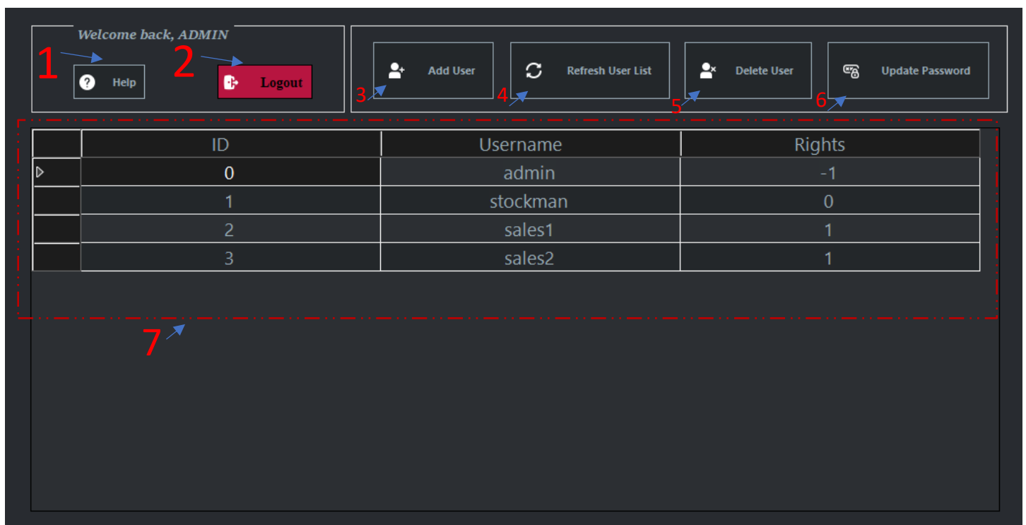
Fig 2. Administrator dashboard
